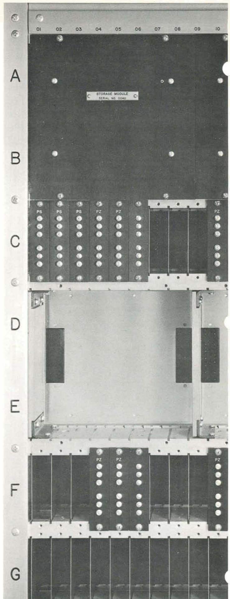
Memory system module installed on the page frame; below, the housing area and connectors into which the memory system module is positioned.
